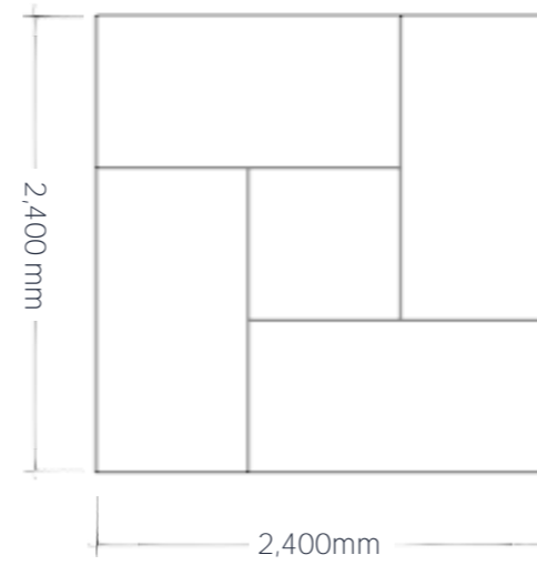
4 table configuration
